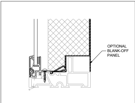
SILL
