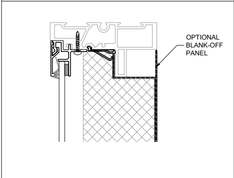
HEAD
