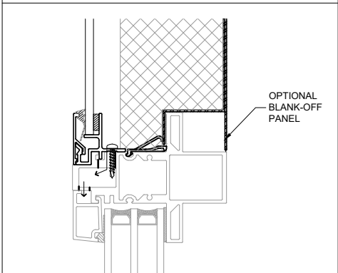
MULLION
