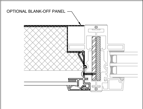
COUPLER
