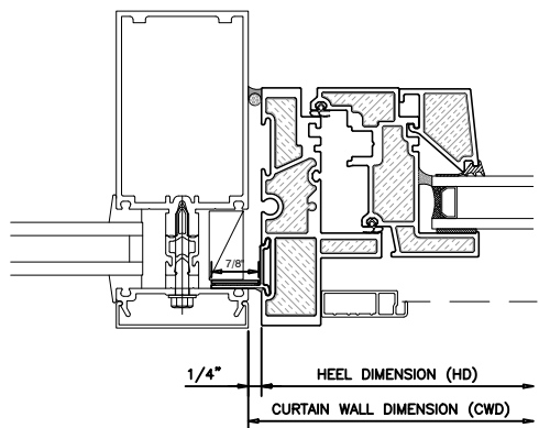
6 OPERABLE JAMB INSWING UNIVERSAL WINDOW
