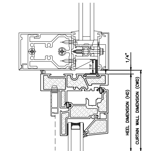
1 OPERABLE HEAD OUTSWING UNIVERSAL WINDOW
