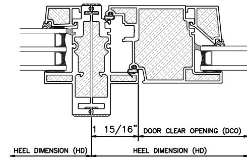
8 VERTICAL COUPLER
