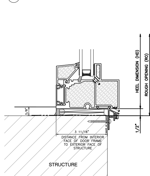
6 SIDELITE FIXED SILL
