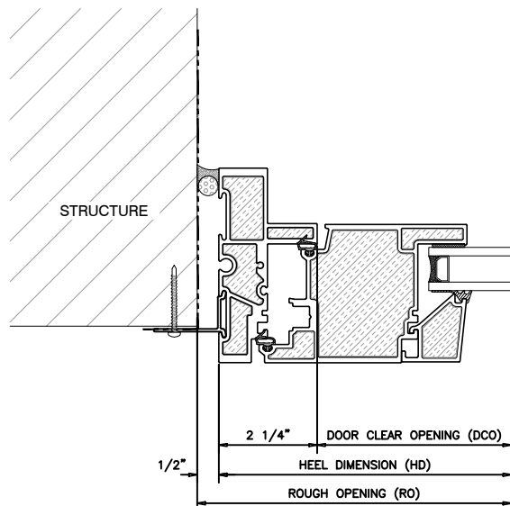
3 OUTSWING DOOR HANDLE JAMB
