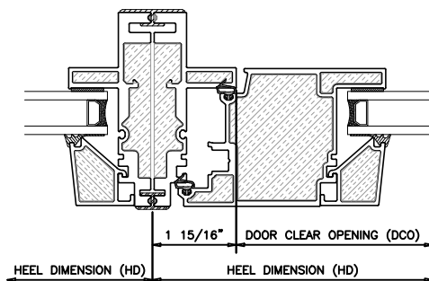
5 VERTICAL COUPLER
