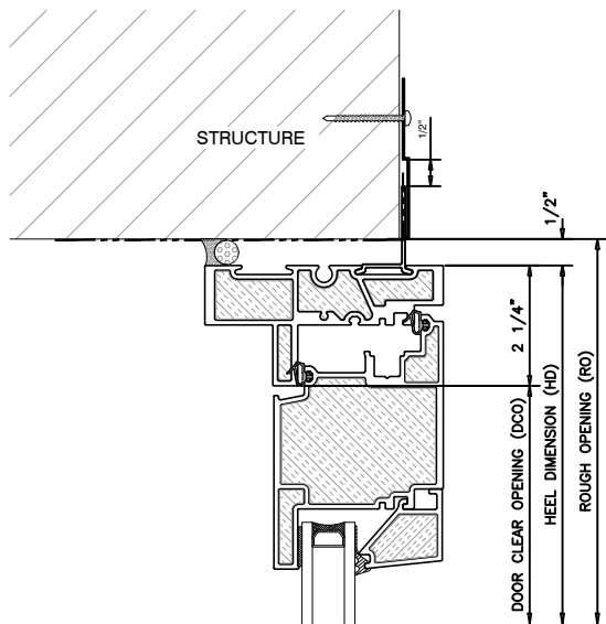
1 OUTSWING DOOR HEAD
