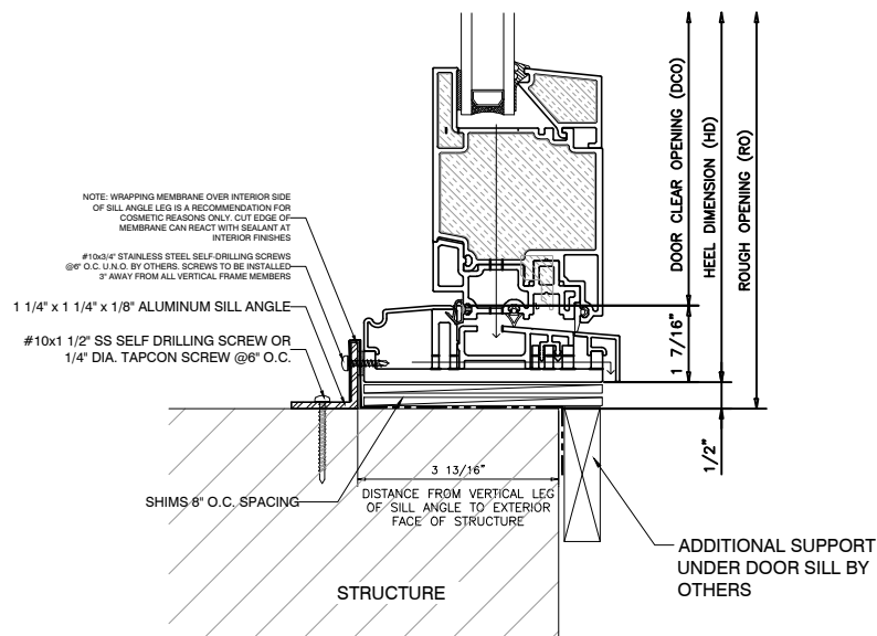
2 OUTSWING DOOR SILL
