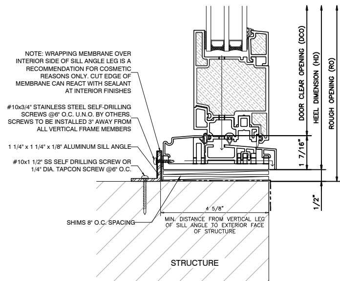
2 OUTSWING DOOR SILL OUTSWING UNIVERSAL DOOR
