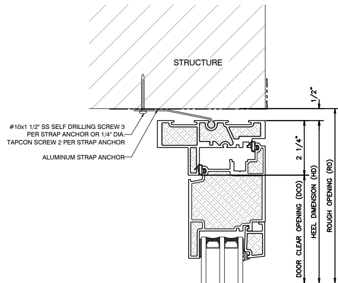
1 OUTSWING DOOR HEAD OUTSWING UNIVERSAL DOOR
