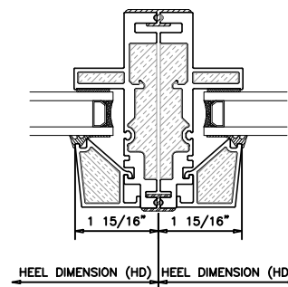
6 VERTICAL COUPLER EXT. GLAZED UNIVERSAL WINDOW
