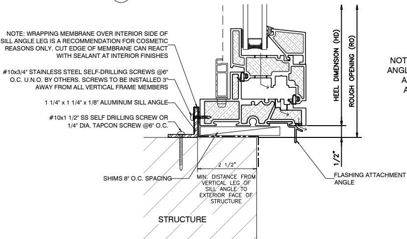
2 OPERABLE SILL OUTSWING UNIVERSAL WINDOW
