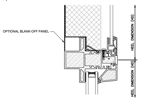
9 HORIZONTAL MULLION @ SPANDREL EXT. GLAZED UNIVERSAL WINDOW
