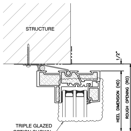
3 FIXED HEAD EXT. GLAZED UNIVERSAL WINDOW
