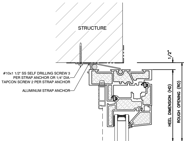
1 OPERABLE HEAD OUTSWING UNIVERSAL WINDOW
