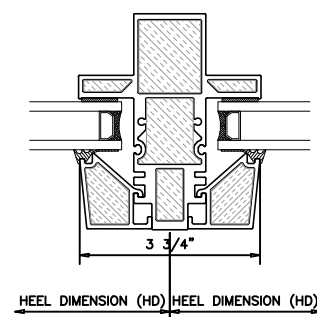
7 VERTICAL MULLION EXT. GLAZED UNIVERSAL WINDOW
