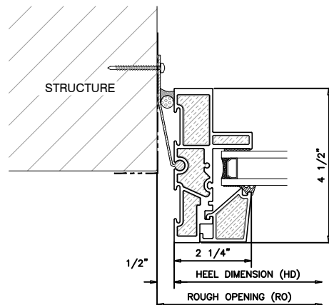
5 FIXED JAMB EXT. GLAZED UNIVERSAL WINDOW
