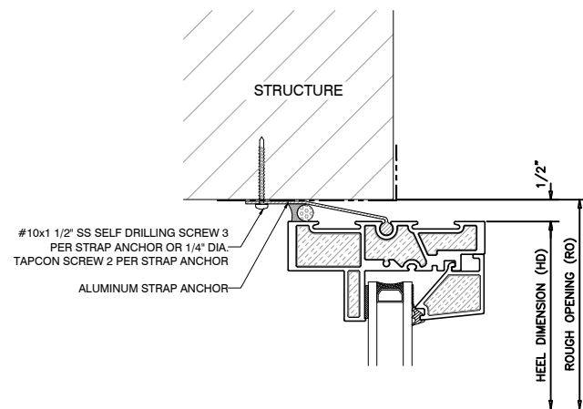
1 FIXED HEAD EXT. GLAZED UNIVERSAL WINDOW
