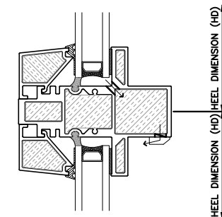
6 HORIZONTAL MULLION INT. GLAZED UNIVERSAL WINDOW
