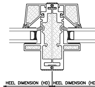
4 VERTICAL COUPLER EXT. GLAZED UNIVERSAL WINDOW
