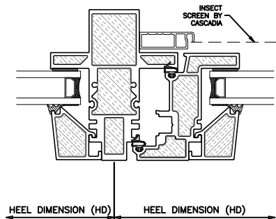
5 VERTICAL MULLION OUTSWING UNIVERSAL WINDOW
