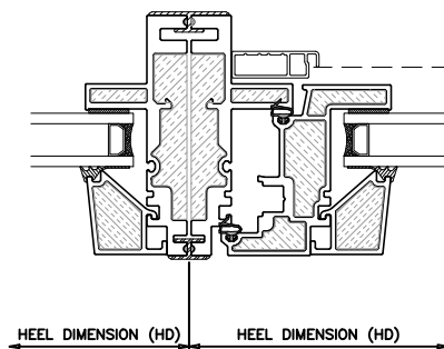
4 VERTICAL COUPLER OUTSWING UNIVERSAL WINDOW
