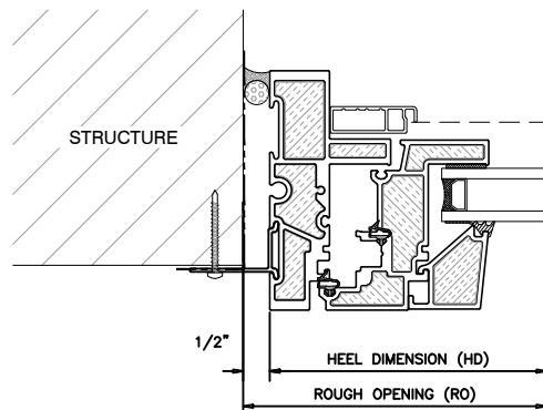
3 OPERABLE JAMB OUTSWING UNIVERSAL WINDOW
