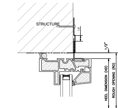
1 FIXED HEAD EXT. GLAZED UNIVERSAL WINDOW
