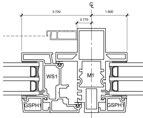
5 MULLION
