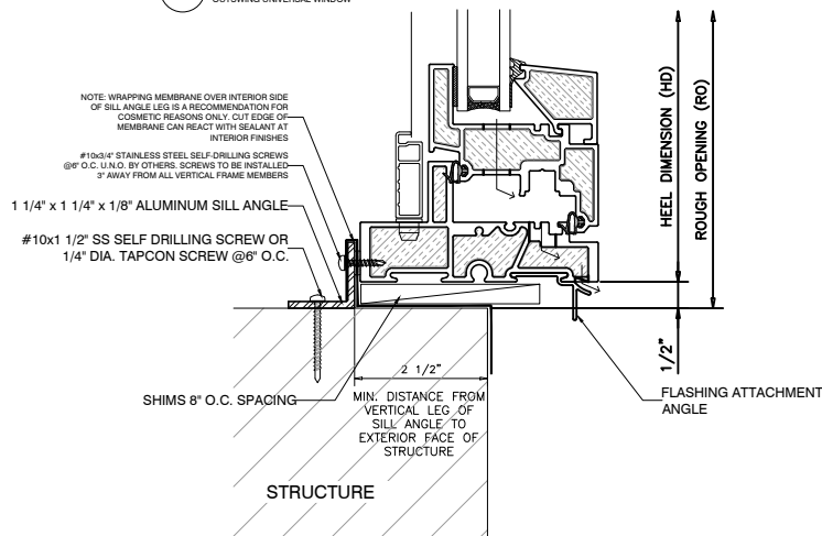
2 OPERABLE SILL OUTSWING UNIVERSAL WINDOW
