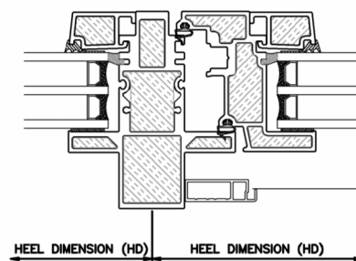
5 VERTICAL MULLION IN SWING UNIVERSAL WINDOW
