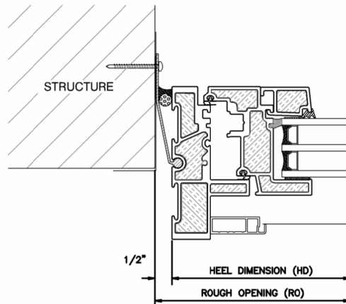
3 OPERABLE JAMB IN SWING UNIVERSAL WINDOW
