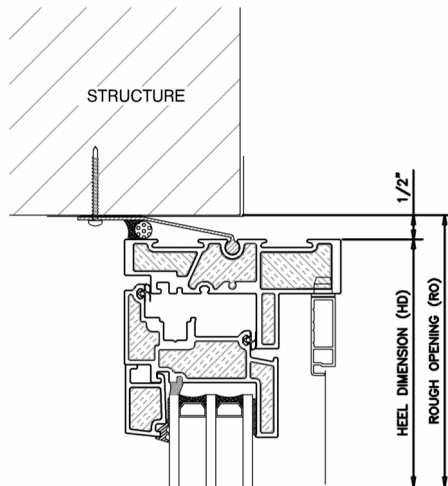
1 OPERABLE HEAD IN SWING UNIVERSAL WINDOW
