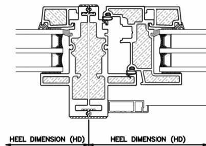
4 VERTICAL COUPLER IN SWING UNIVERSAL WINDOW
