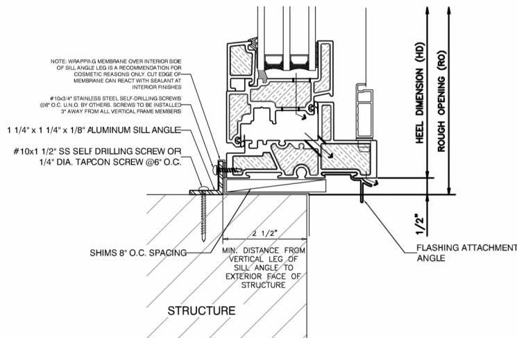
2 OPERABLE SILL IN SWING UNIVERSAL WINDOW
