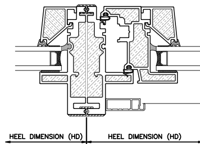
4 VERTICAL COUPLER INSWING UNIVERSAL WINDOW
