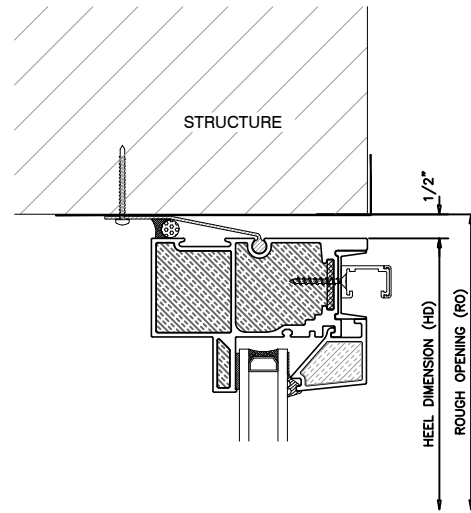
3 SLIDE-OUT FIXED HEAD OUTWARD SLIDING DOOR
