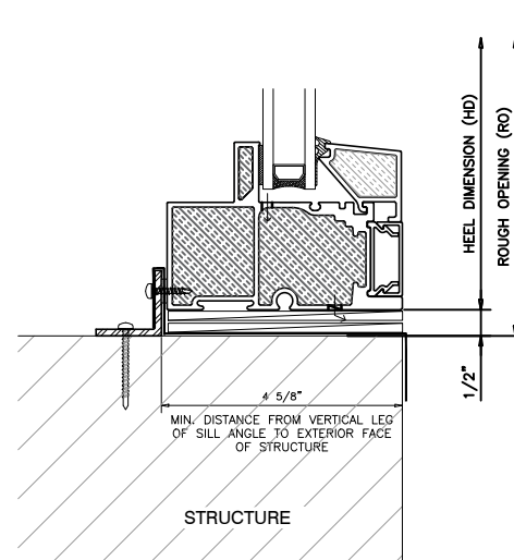
6 SIDELITE FIXED SILL OUTWARD SLIDING DOOR
