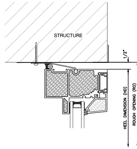
5 SIDELITE FIXED HEAD OUTWARD SLIDING DOOR
