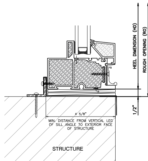
4 SLIDE-OUT FIXED SILL OUTWARD SLIDING DOOR
