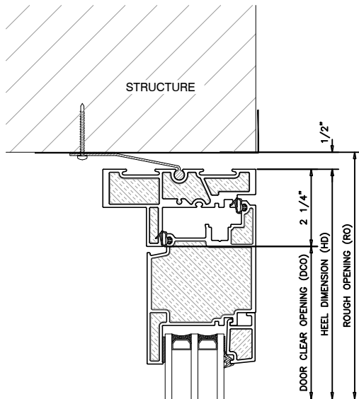
1 OUTSWING DOOR HEAD OUTSWING UNIVERSAL DOOR
