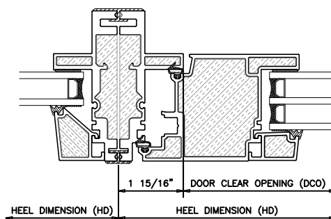
5 VERTICAL COUPLER OUTSWING UNIVERSAL DOOR
