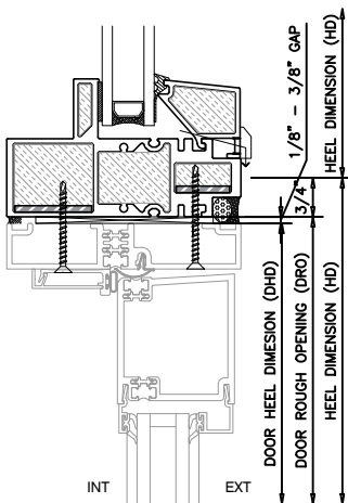
2 DOOR HEAD @ TRANSOM EXT. GLAZED UNIVERSAL - INSERT BY OTHERS
