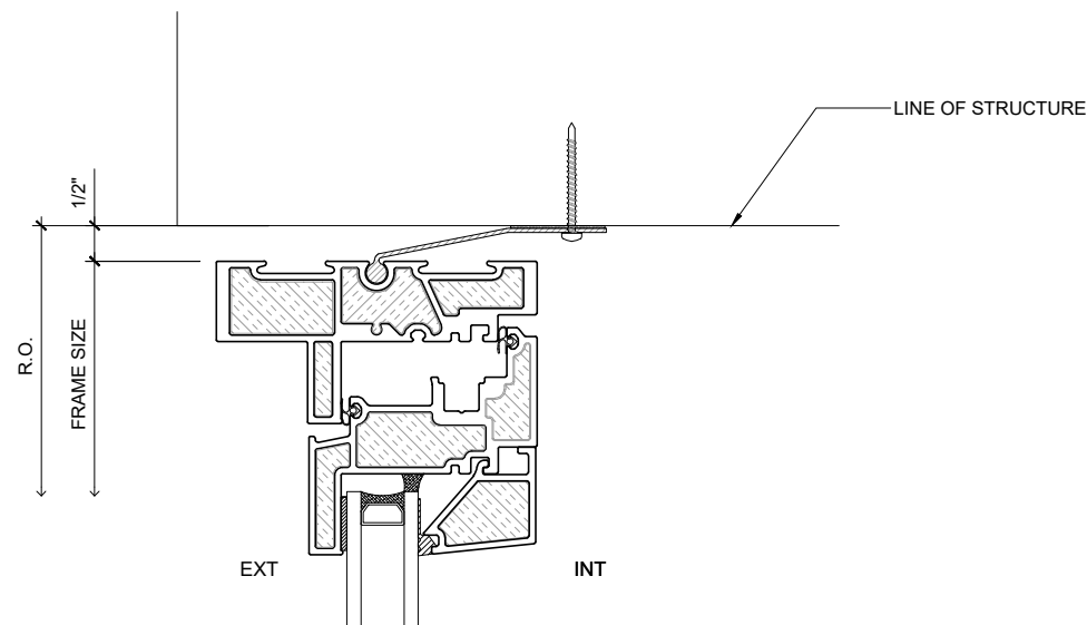
D OPERABLE HEAD H1 SCALE: 4"=1'-0"
