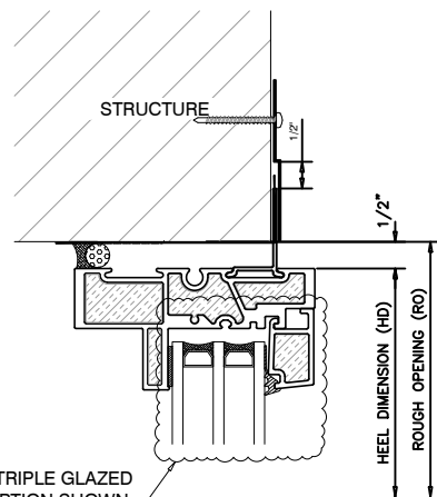
3 FIXED HEAD EXT. GLAZED UNIVERSAL WINDOW
