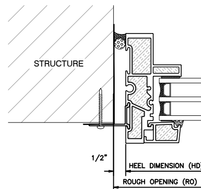
5 FIXED JAMB EXT. GLAZED UNIVERSAL WINDOW
