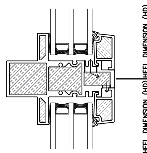
8 HORIZONTAL MULLION EXT. GLAZED UNIVERSAL WINDOW
