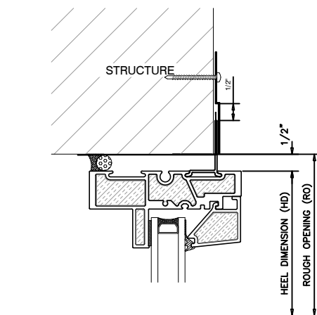
1 FIXED HEAD EXT. GLAZED UNIVERSAL WINDOW
