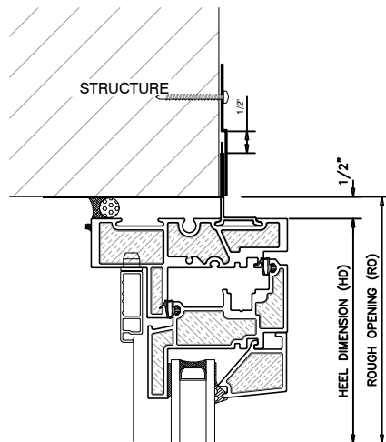
1 OPERABLE HEAD OUTSWING UNIVERSAL WINDOW
