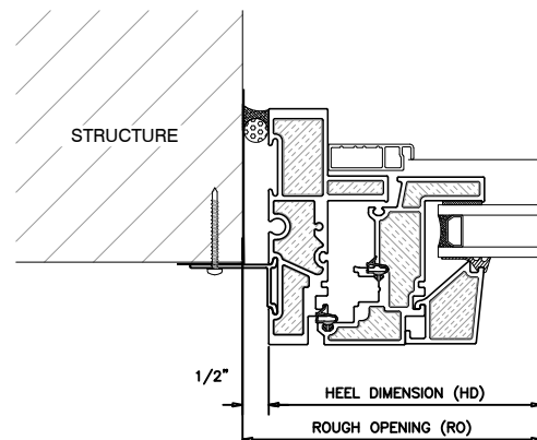
3 OPERABLE JAMB OUTSWING UNIVERSAL WINDOW
