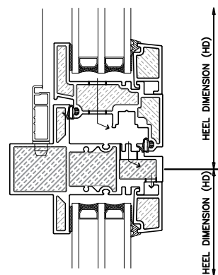
6 HORIZONTAL MULLION OUTSWING UNIVERSAL WINDOW
