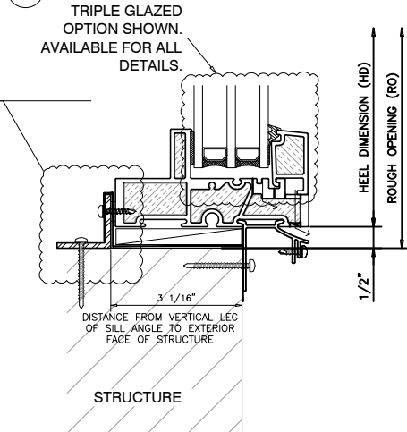
4 FIXED SILL EXT. GLAZED UNIVERSAL WINDOW
