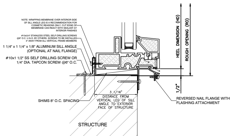
2 FIXED SILL EXT. GLAZED UNIVERSAL WINDOW
