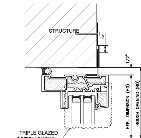
3 FIXED HEAD EXT. GLAZED UNIVERSAL WINDOW
