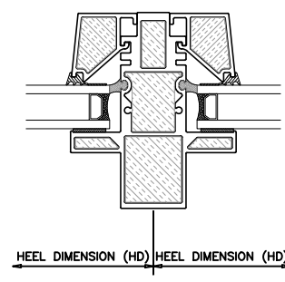
5 VERTICAL MULLION INT. GLAZED UNIVERSAL WINDOW
