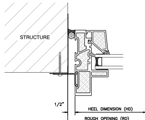
3 FIXED JAMB INT. GLAZED UNIVERSAL WINDOW
