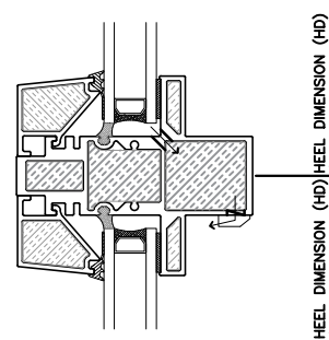
6 HORIZONTAL MULLION INT. GLAZED UNIVERSAL WINDOW
