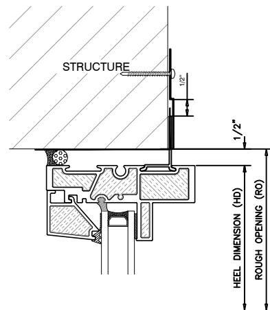
1 FIXED HEAD INT. GLAZED UNIVERSAL WINDOW
