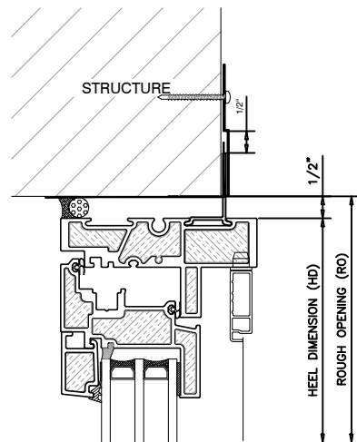
1 OPERABLE HEAD INSWING UNIVERSAL WINDOW
