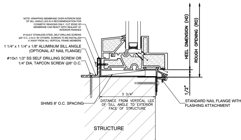
2 FIXED SILL INT. GLAZED UNIVERSAL WINDOW
