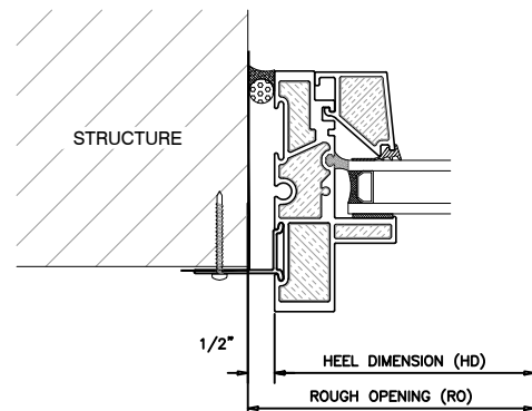
3 FIXED JAMB INT. GLAZED UNIVERSAL WINDOW
