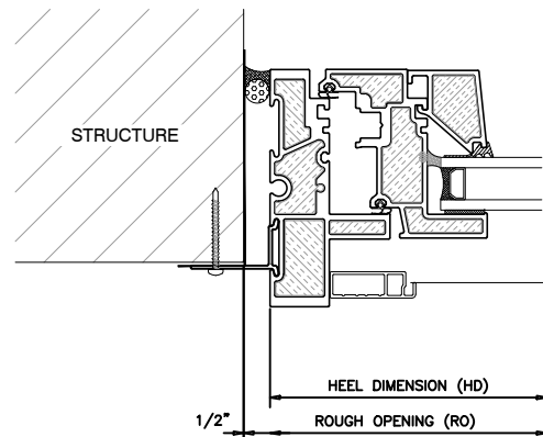
3 OPERABLE JAMB INSWING UNIVERSAL WINDOW
