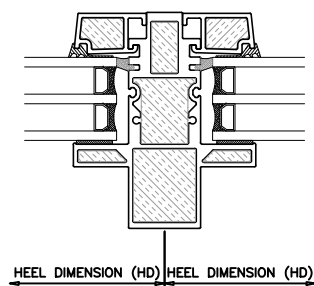
5 VERTICAL MULLION INT. GLAZED UNIVERSAL WINDOW
