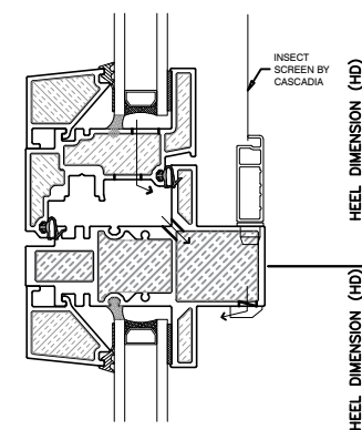
6 HORIZONTAL MULLION INSWING UNIVERSAL WINDOW
