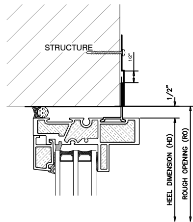
1 FIXED HEAD INT. GLAZED UNIVERSAL WINDOW
