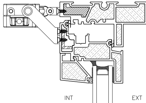
5 MOTORIZED OPERATOR @ HOPPER HEAD INSWING UNIVERSAL WINDOW
