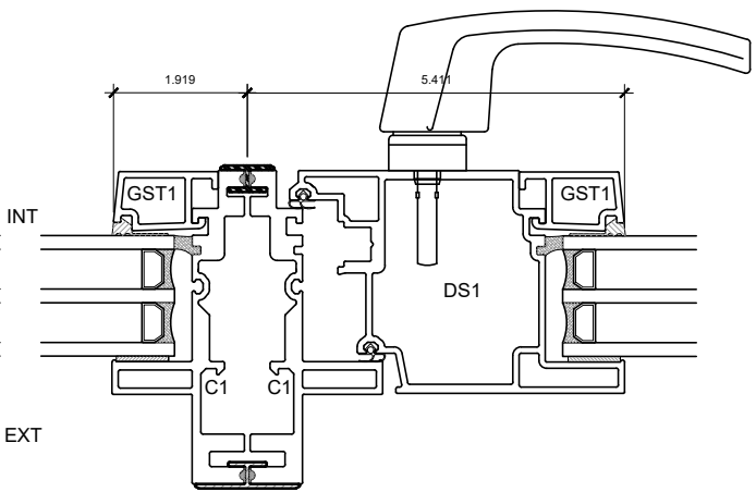
4 COUPLED MULLION
