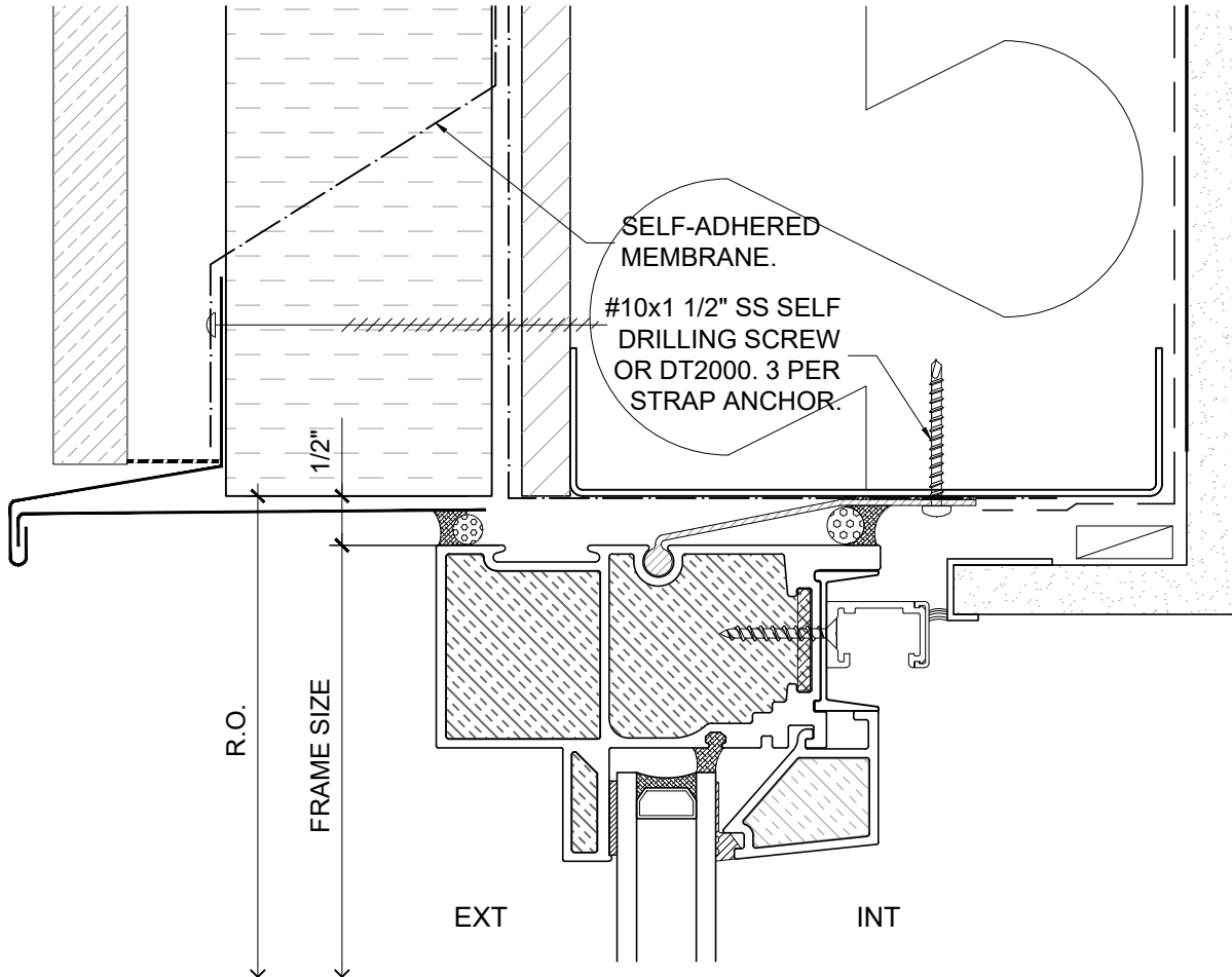
DOUBLE GLAZED SLIDE-IN DOOR SIDELITE
