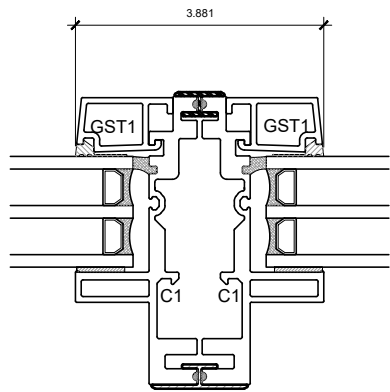
5 COUPLED MULLION
