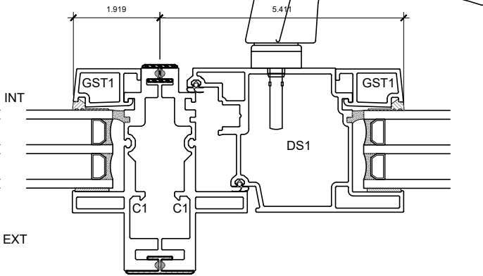
4 COUPLED MULLION
