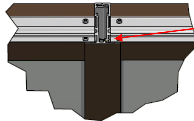
DETAIL D SCALE 0.40 : 1
